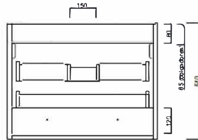
BACK ELEVATION
